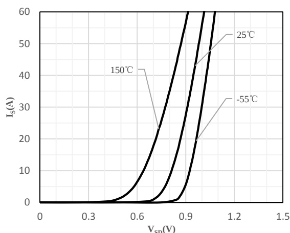
Fig 6 Body-Diode Characteristics
